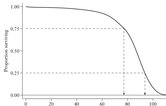
Figure 3.4 An \ell_x curve
